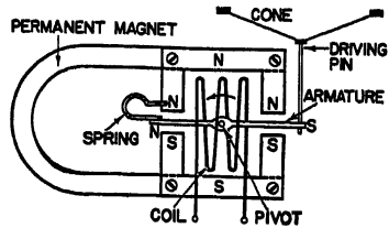
Examples and operating principle of balanced-armature magnetic loudspeakers.
